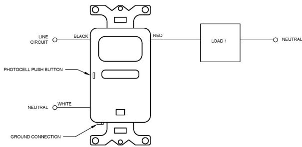
SINGLE POLE WIRING
