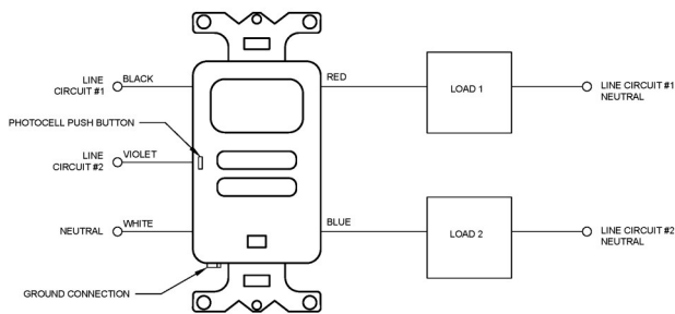
TWO POLE WIRING
