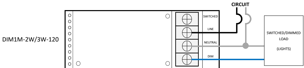
WIRING – 2-WIRE — INSTALLED ON RIGHT SIDE OF RD-32-S2
