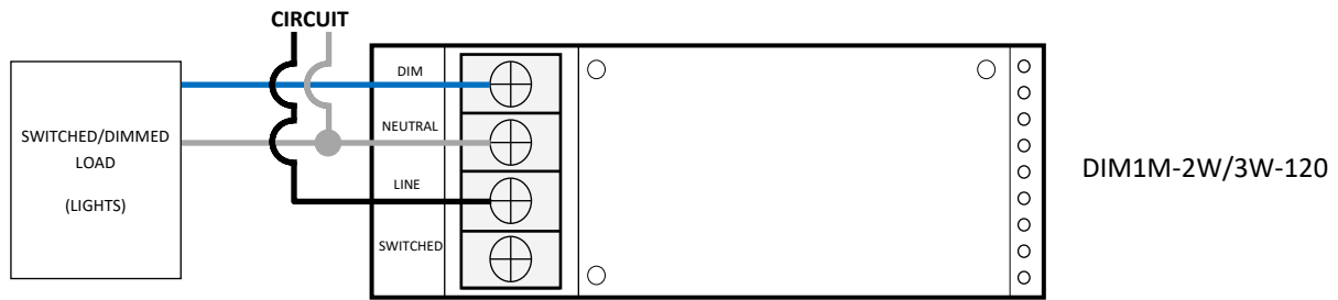
WIRING – 2-WIRE — INSTALLED ON LEFT SIDE OF RD-32-S2
