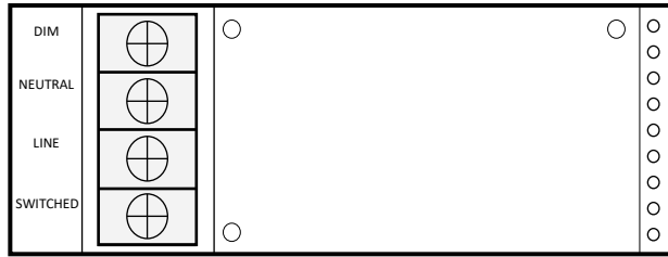
DIM1M-2W/3W-120 (ENLARGED FOR CLARITY)
