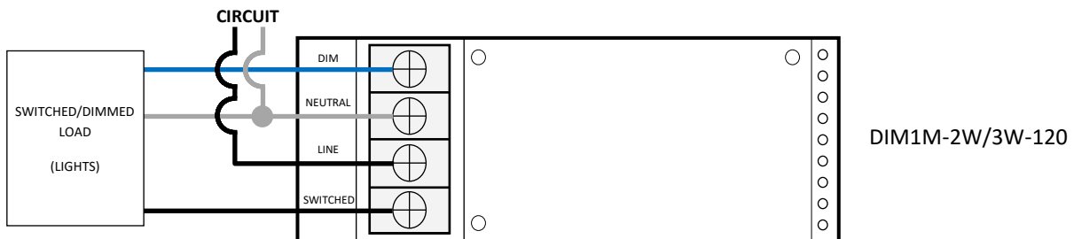
WIRING – 3-WIRE — INSTALLED ON LEFT SIDE OF RD-32-S2
