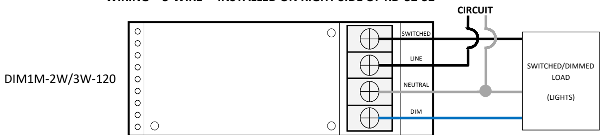
WIRING – 3-WIRE — INSTALLED ON RIGHT SIDE OF RD-32-S2
